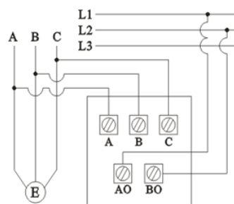
Synchronoscope
